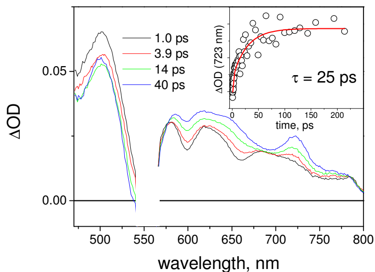
Figure 6. Ultrafast spectroscopy of SnRu 2 in CH 2 Cl 2 (excitation at 555 nm). Inset: Kinetic analysis at 725 nm.
