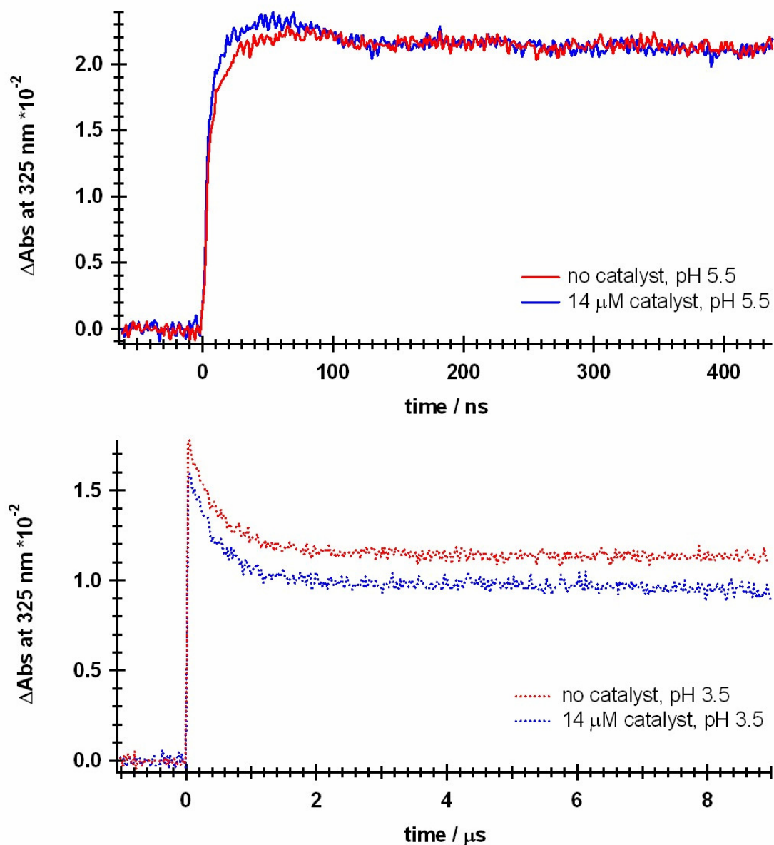
Figure 3. ^*\text{[Ru(bpy)}_3\text{]}^{2+} transient absorption traces at 325 nm at high (top panel) and low pH (lower panel). 13-15 \mu\text{M} [\text{Ru(bpy)}_3]^{2+} , 100 mM ascorbic acid, 1:1 DMF/ \text{H}_2\text{O} , room temperature. Excitation at 470 nm.
