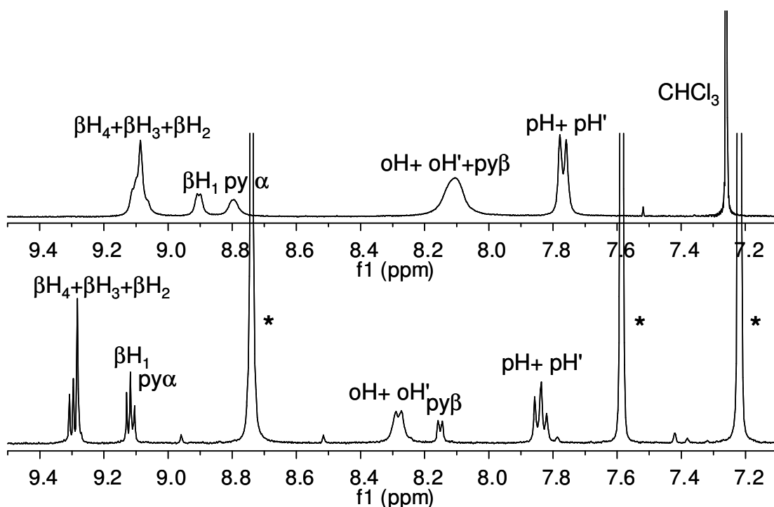
Figure 2. Aromatic region of the ^1\text{H} NMR of AIMPyP in \text{CDCl}_3 , top, and pyridine- d_5 , bottom. See AIMPyP part of Scheme 2 for proton labels. Peaks of residual non-deuterated pyridine are indicated with an asterisk.
