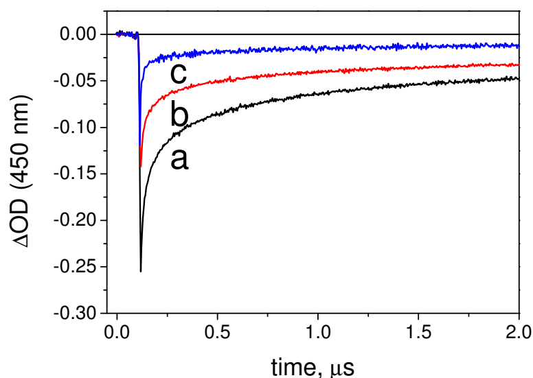
Figure 2. Laser flash photolysis (excitation, 532 nm, FWHM 8ns) of a nanocrystalline TiO 2 layer sensitized with Ru(bpy) 2 (dpb) 2+ ( 8 \times 10^{-8} mol/cm 2 ). As such (a), and loaded with 6.6 \times 10^{-9} mol/cm 2 1 (b) or 3.2 \times 10^{-8} mol/cm 2 1 (c).
