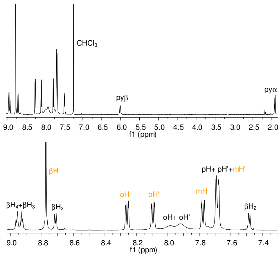
Figure 3. ^1\text{H} NMR ( \text{CDCl}_3 ) of AIMPyP-RuP (top, tert -butyl groups omitted for clarity) and its enlarged aromatic region (bottom). See Scheme 2 for proton labels.
