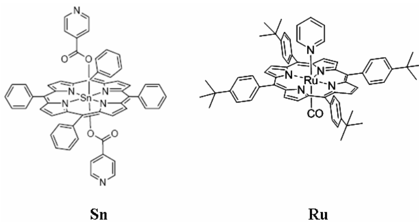
Chart 2. Structural formulas of the monomeric model compounds Sn and Ru .
