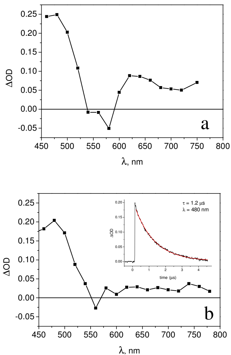
Figure 8. Nanosecond laser flash photolysis of \text{SnRu}_2 , \lambda_{\text{xc}} = 532 nm. (a) \text{CH}_2\text{Cl}_2 , differential absorption spectrum recorded at the maximum of the excitation pulse. (b) Toluene, differential absorption spectrum recorded at 50 ns delay time; inset, kinetic analysis at 480 nm.
