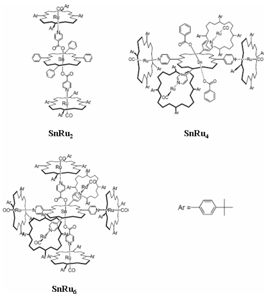
Chart 1. Structural formulas of the arrays studied.
