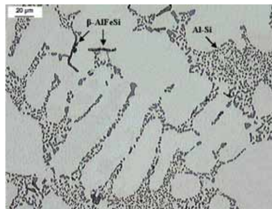
Fig. 5. Optical micrograph showing secondary phase particles in rim area of wheel-3. The distribution of eutectic silicon is homogeneous and globular.
