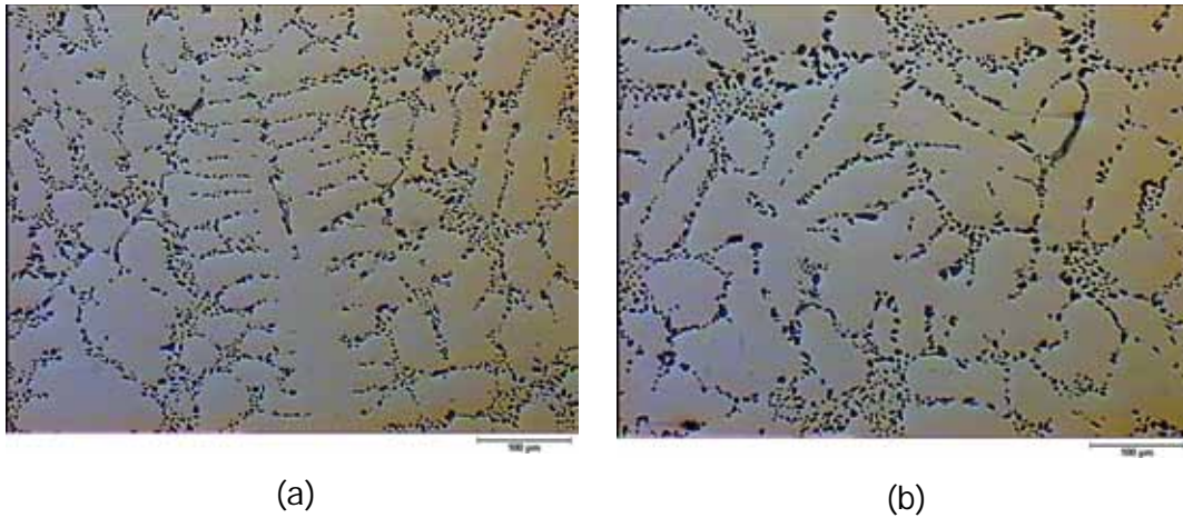
Fig. 3. Microstructure of a casting realised with full cores: a) position 1, b) position 2.
