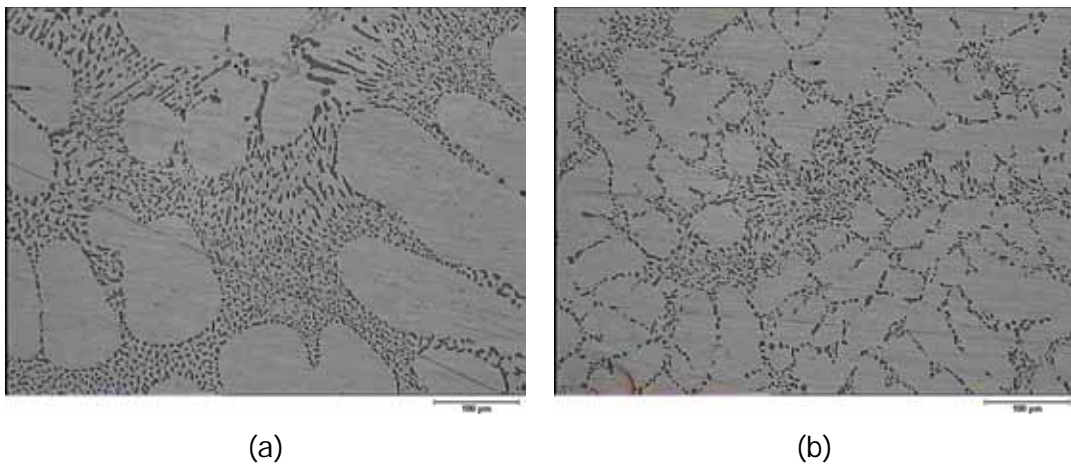
Fig. 5. Microstructure A356 Na-modified alloy: a) un-chilled, b) chilled.
