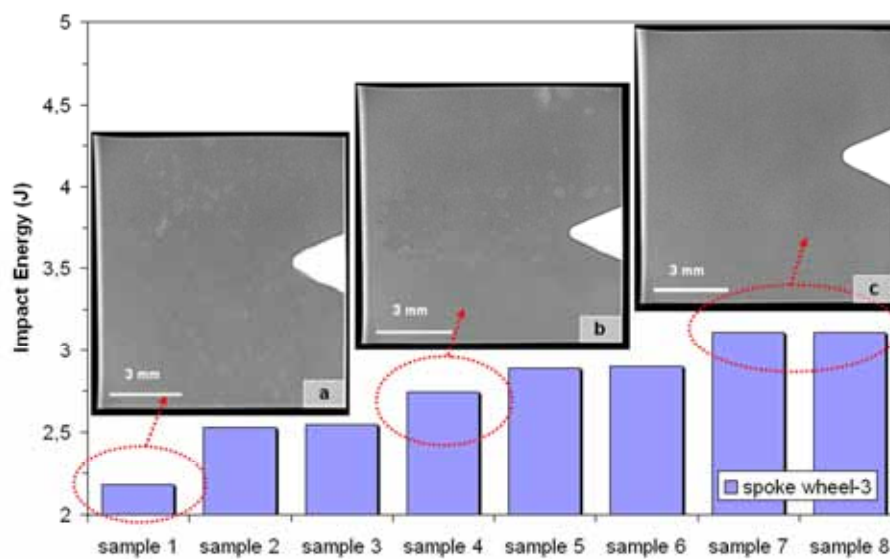
Fig. 15. Impact energy of some samples drawn from the spoke of wheel-3 associated with respective X-ray images, taken in the zone around the V-notch. The X-ray images refer to a high (a), medium (b) and low (c) defect content.
